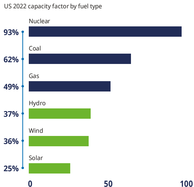
Figure 17: Capacity factor of energy sources is an important determinant of competitiveness, and is captured in LCOE estimates
